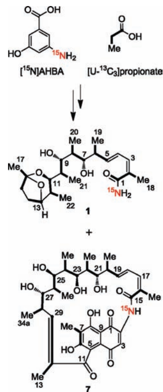
Figure 4. Stable isotope labeling pattern observed for 1 and proposed for 7 (see ref 43) from the incorporation of [ 15 N]AHBA and [U- 13 C 3 ]propionate.
