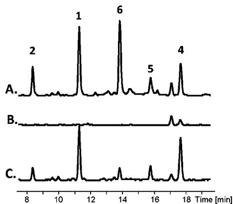
Figure 3. HPLC-MS analysis of the inactivation of the S. arenicola AHBA synthase ( rifK , sareI255 ) and chemical complementation of resulting mutant ( rifK::apr R ). Extracted ion chromatogram (EIC) for masses corresponding to the m/z of the sodium adducts of the saliniketals (1–2) and rifamycins (4–6) from Salinispora arenicola (A) wild-type, (B) rifK::apr R , and (C) rifK::apr R mutant chemically complemented with synthetically prepared AHBA (25 mM).
